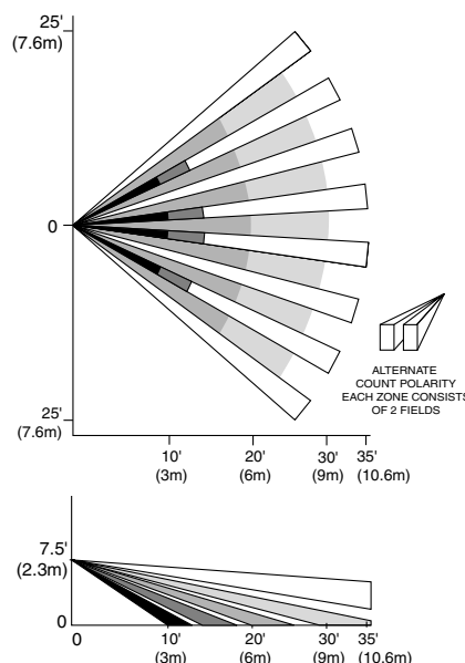
Figure 1. Protection Pattern
