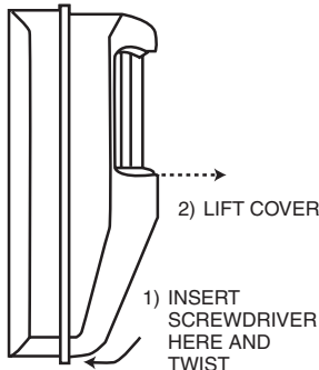
Figure 2. Cover Removal
